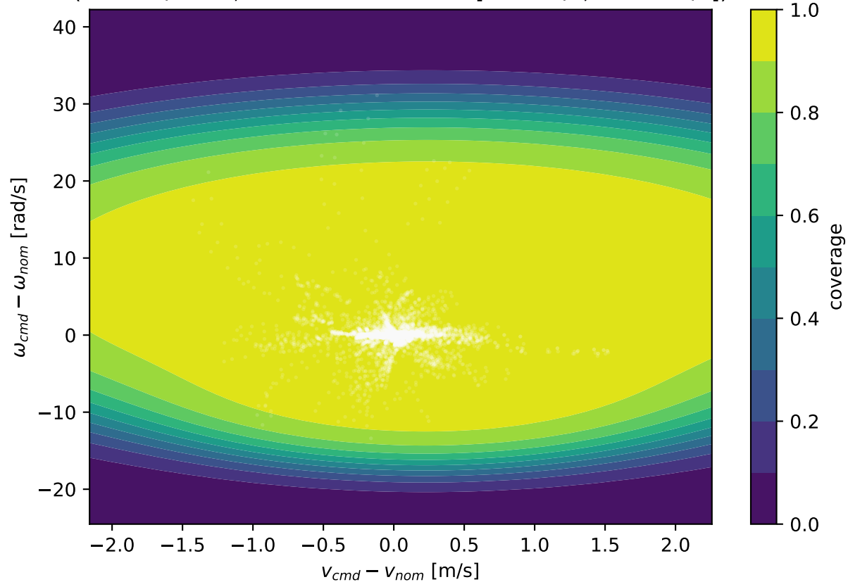
Residual coverage vs command offset (0 = off / OOD; state fixed at mean [0.37 m/s, 0.03 rad/s])
